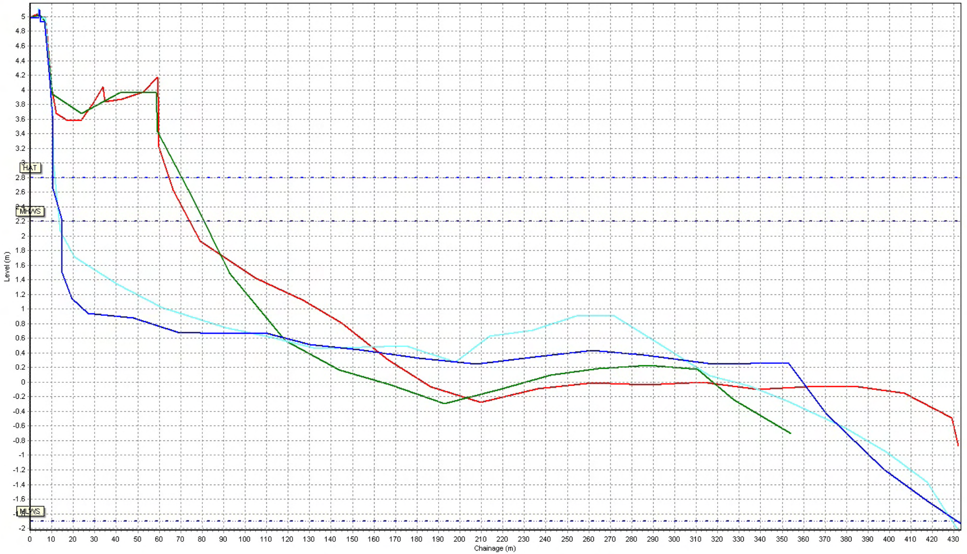
Beach Profiles: 1aBTBC04
