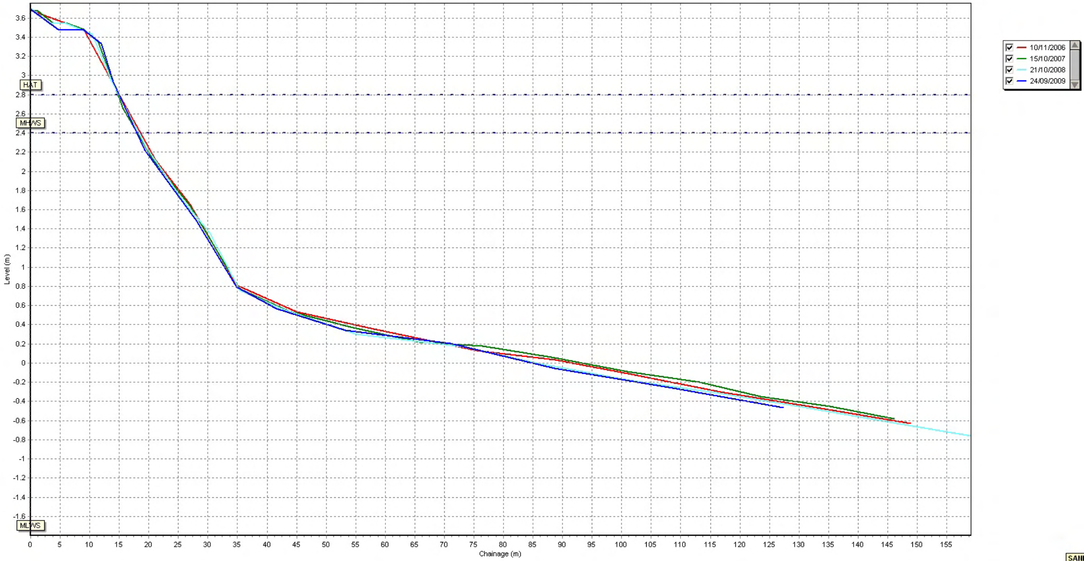
Beach Profiles: 1aBTBC26
