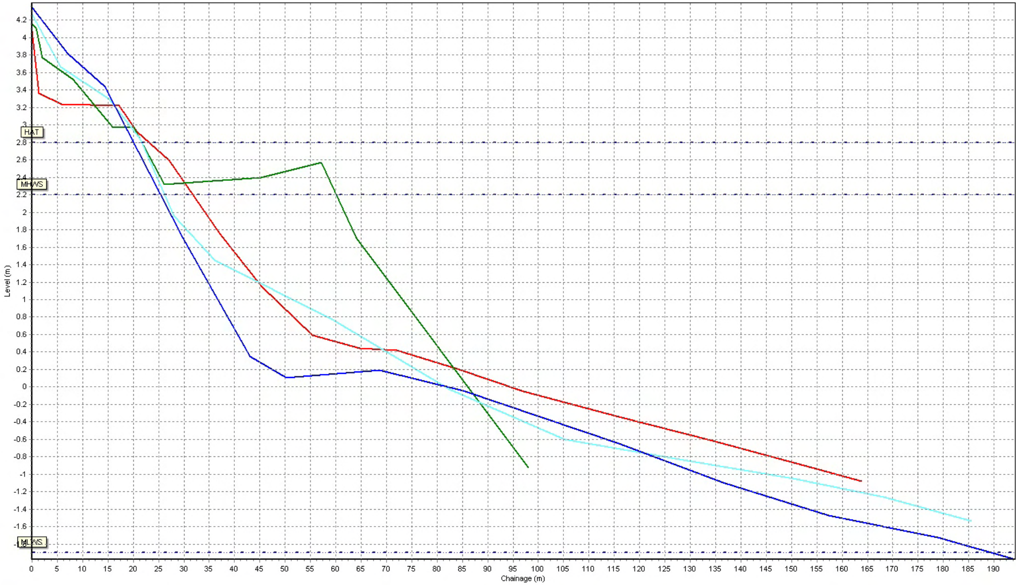
Beach Profiles: 1aBTBC12
