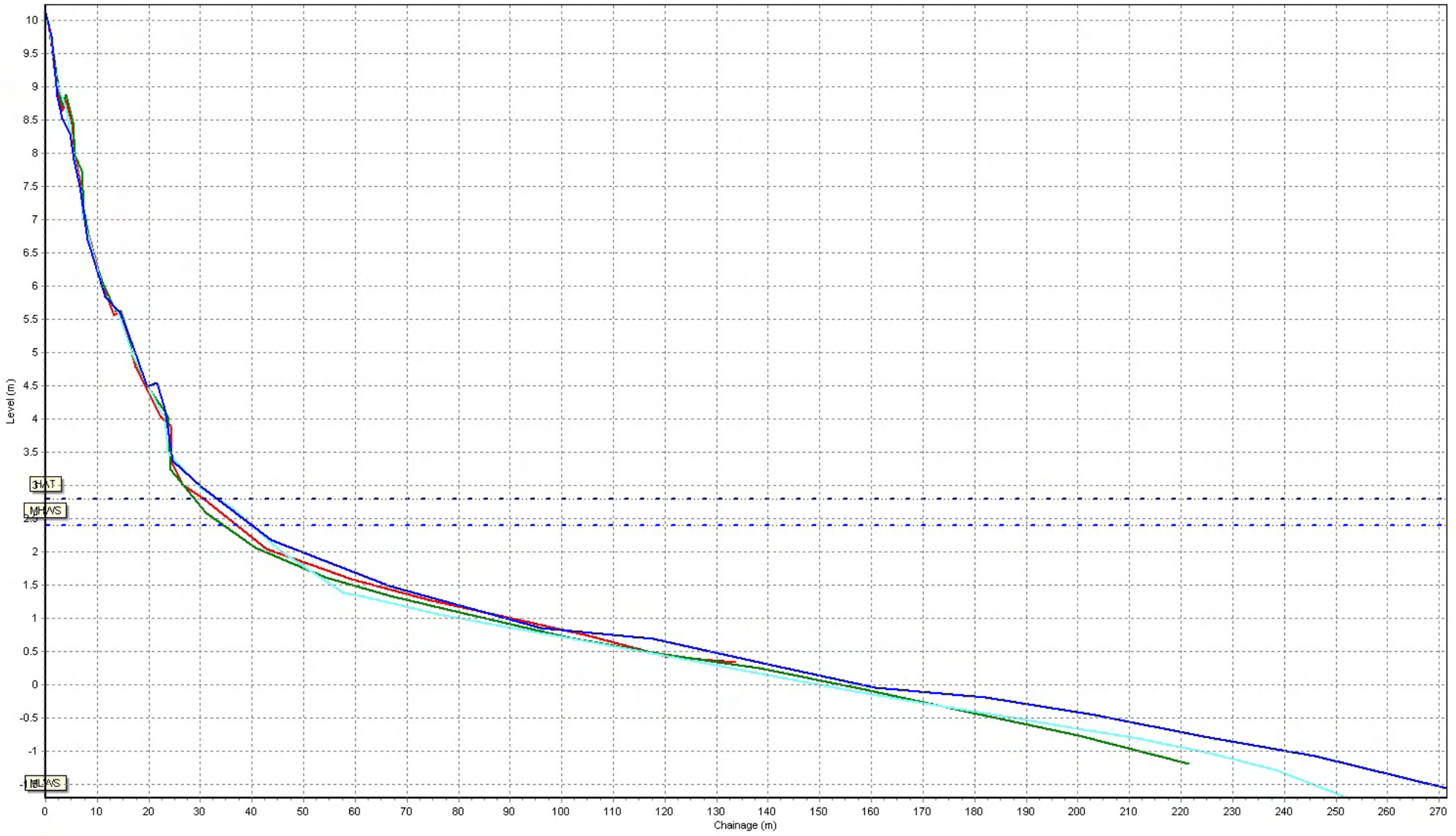
Beach Profiles: 1aBTBC36
