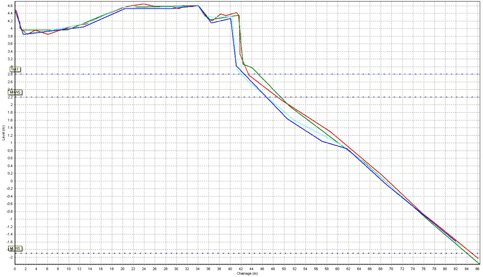
Beach Profiles: 1aBTBC02
