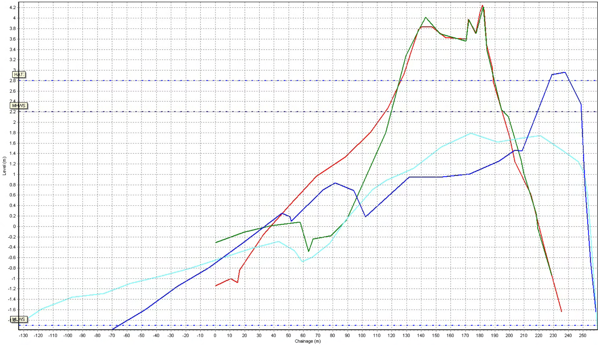
Beach Profiles: 1aBTBC05
