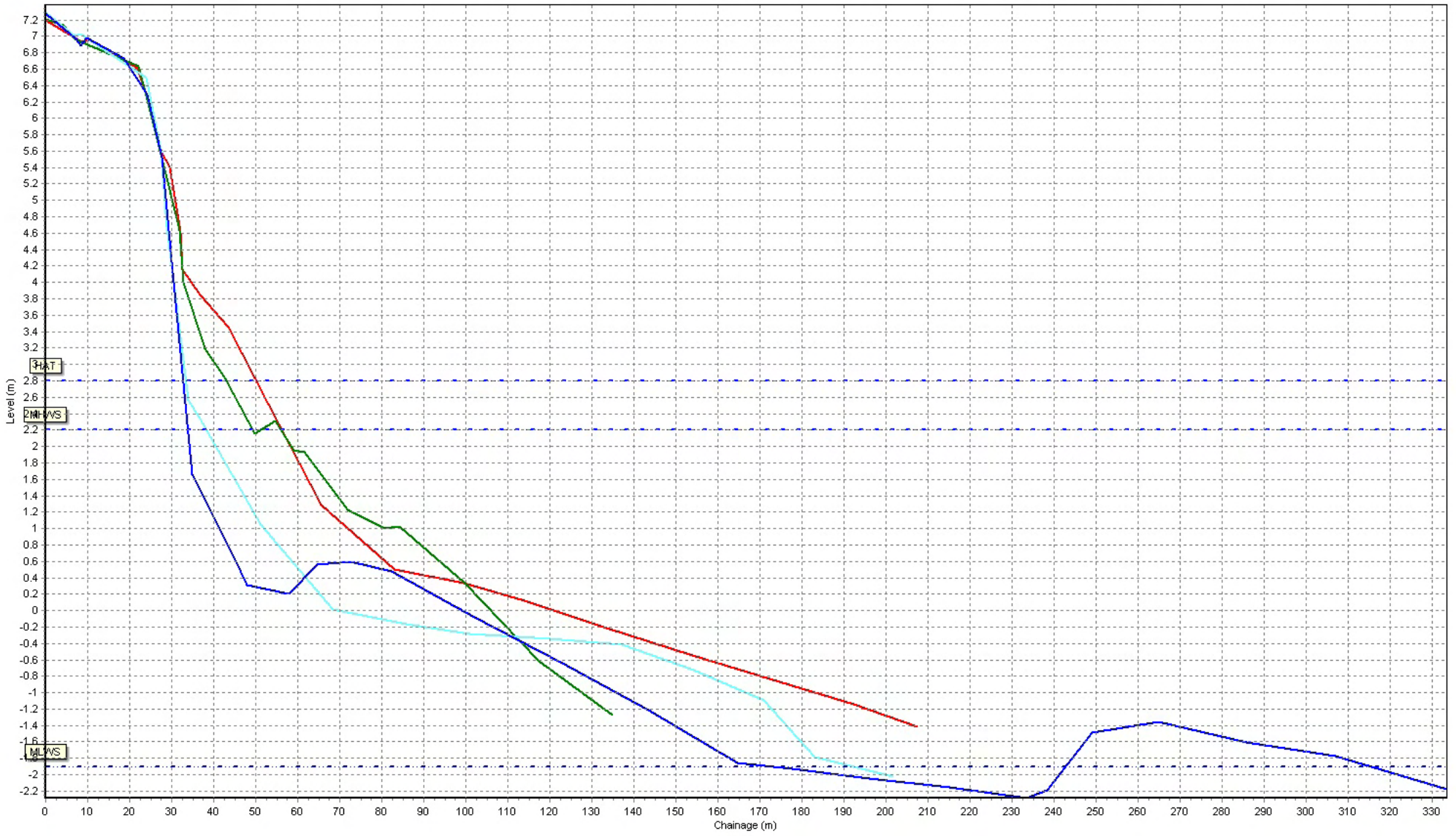
Beach Profiles: 1aBTBC08
