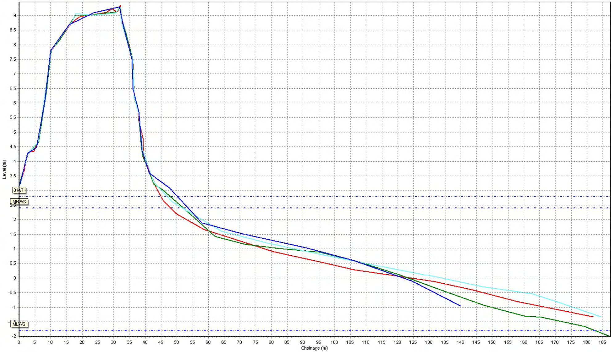
Beach Profiles: 1aBTBC16
