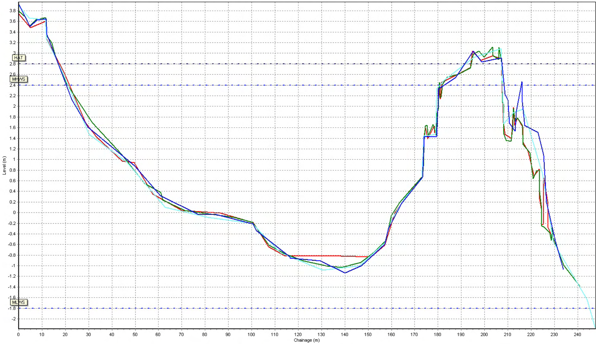
Beach Profiles: 1aBTBC27
