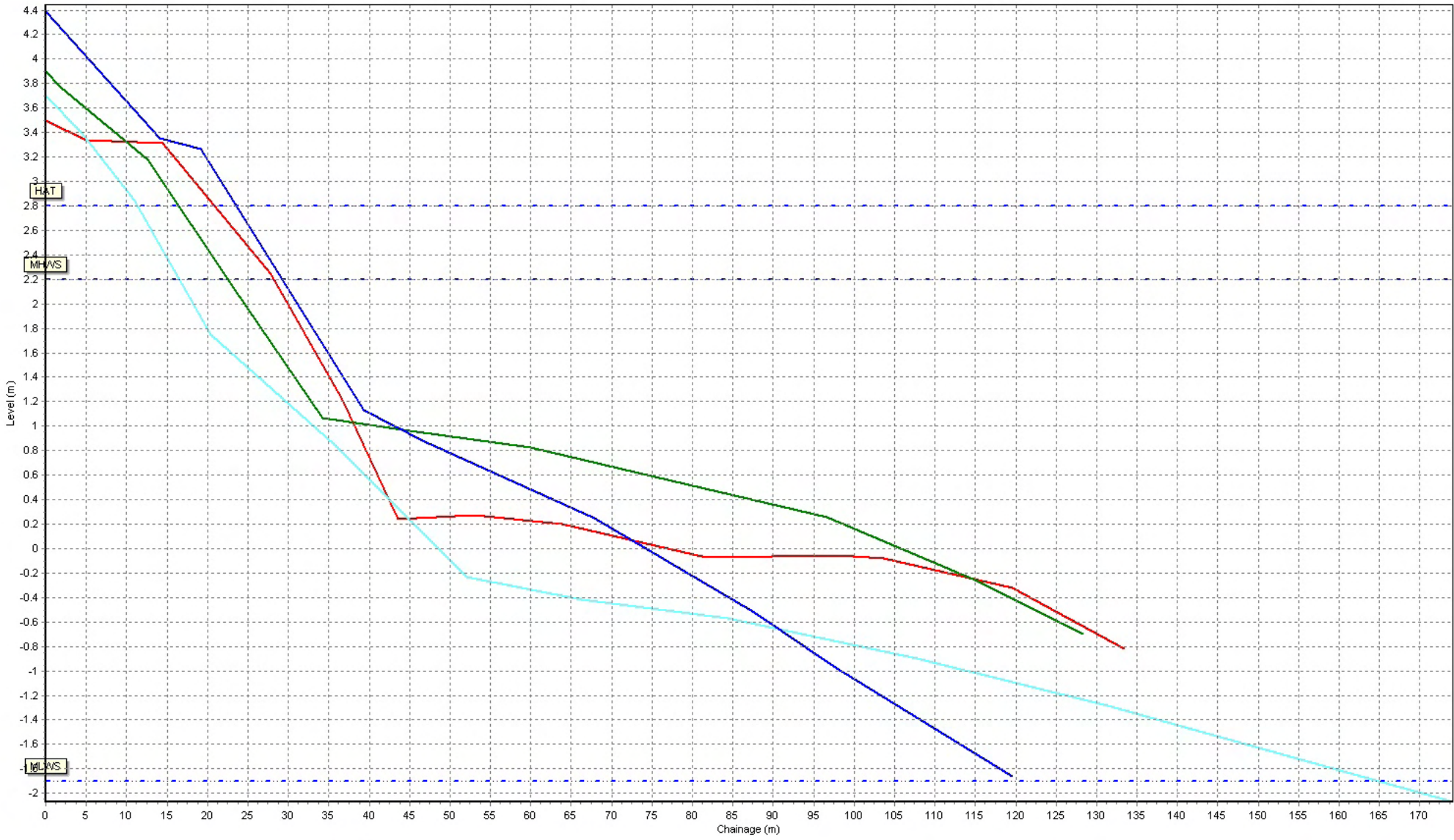
Beach Profiles: 1aBTBC13
